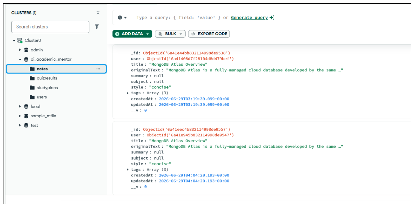
Figure : Notes Collection
